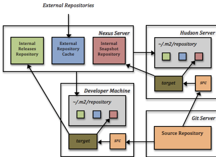
Figure 10. Maven Registry Architecture
