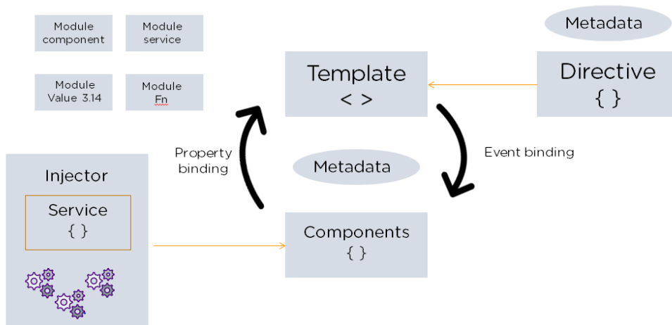
Figure 20. Angular Building Architecture
