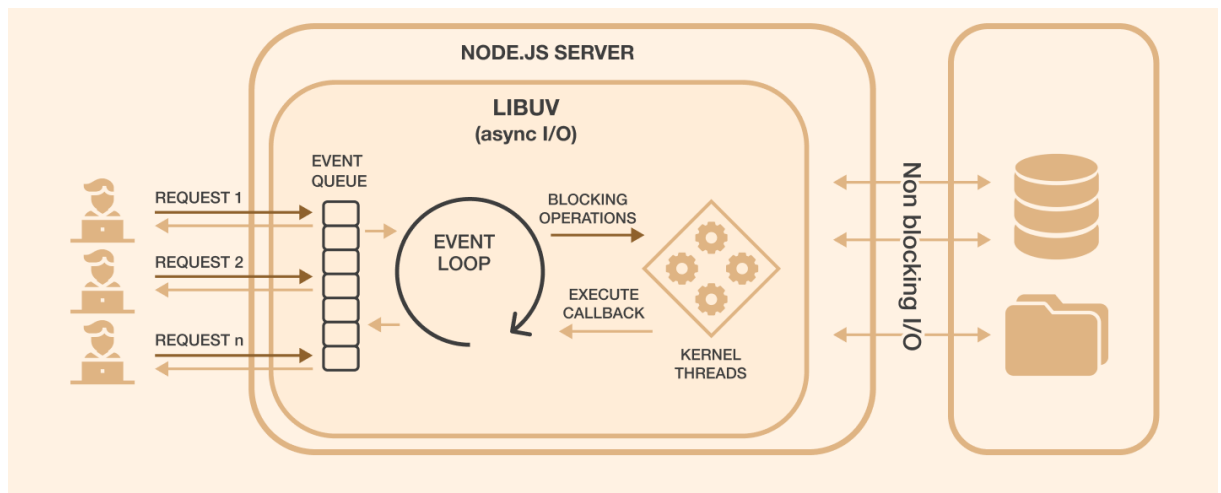
Figure 16. NodeJS Server Architecture
