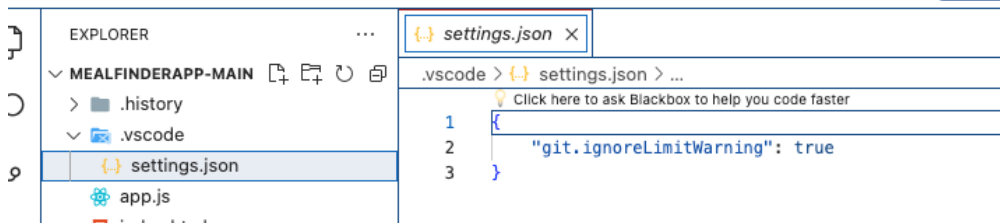
Figure 4. Json Format
