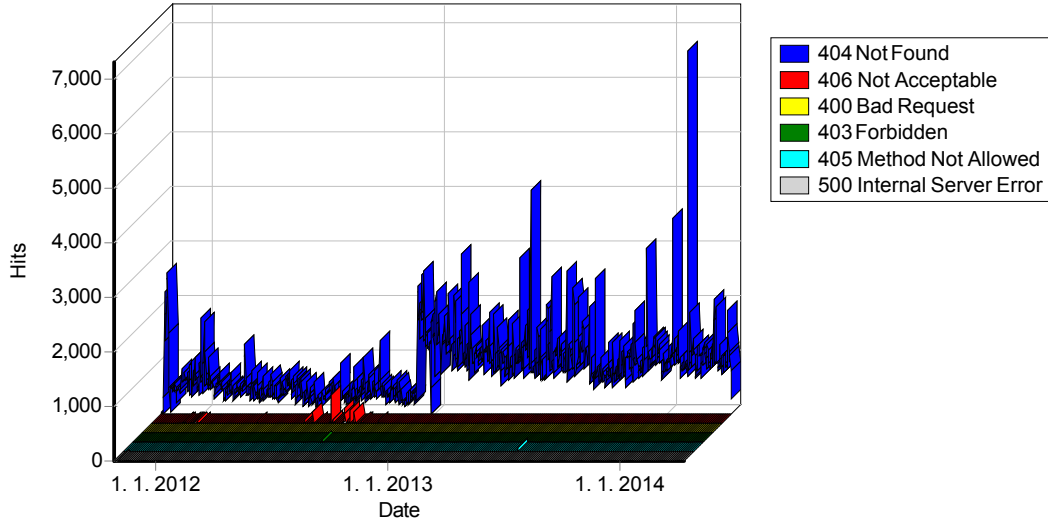
Error Types
