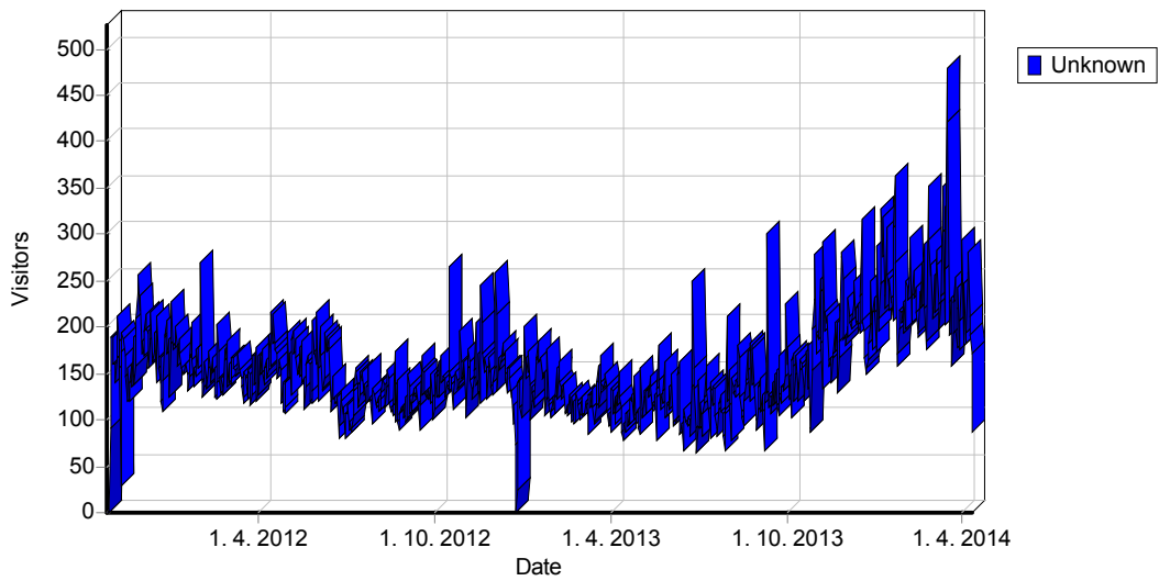
Top-Level Domains
