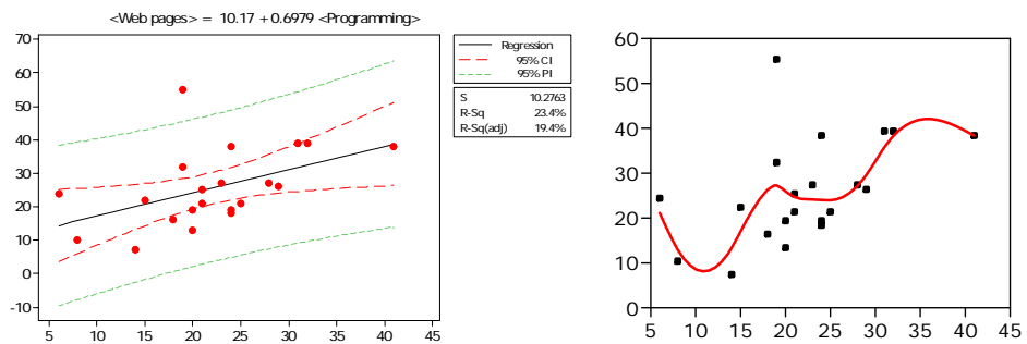
(b) Linear regression model with 95% confidence and prediction interval (c) Spline fit smoothing at \lambda = 10
