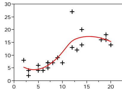
(c) Spline fit smoothing at \lambda = 10
