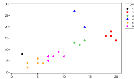
(g) K-Means clustering: standardise variables, 6 clusters
